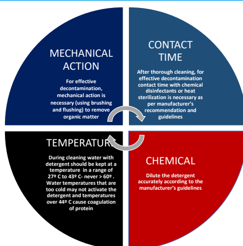
Fig 5.5 The Sinner cycle for cleaning of instruments (Dr Herbert Sinner, 1959).
